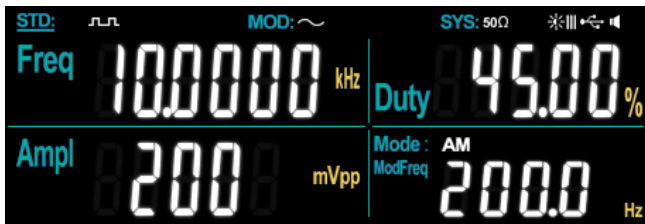
Picture 4-6 Set AM carrier parameters
