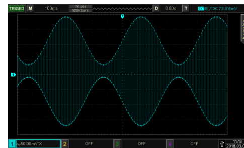
Picture 4-8 AM output waveform
