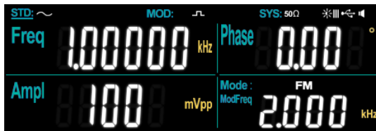
Picture 4-13 Set FM carrier waveform
