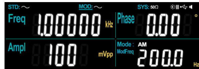
Picture 4-4 Set AM modulation frequency
